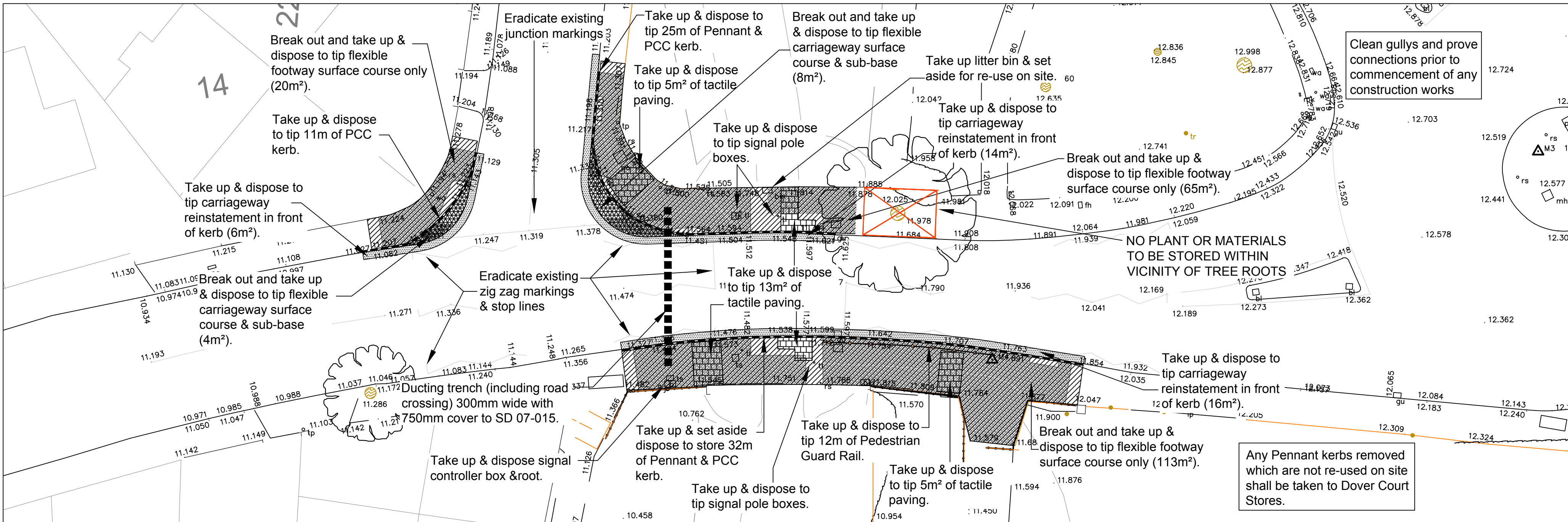
SITE CLEARANCE PLAN 1:200 @A1
